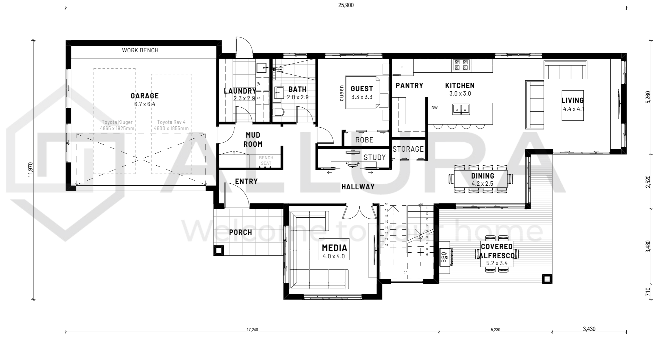
1 GROUND FLOOR PLAN 1:100
