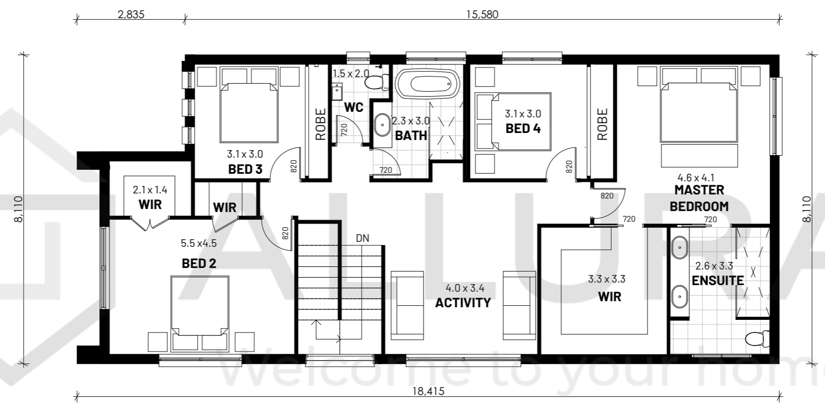
1 FIRST FLOOR PLAN 1:100
