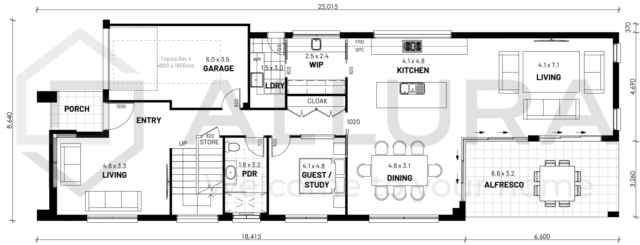
1 GROUND FLOOR PLAN - 1:100
